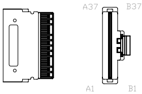
CN1 SFF-8654 SLIMLINE 74M 8i (5XPL-386-E)
